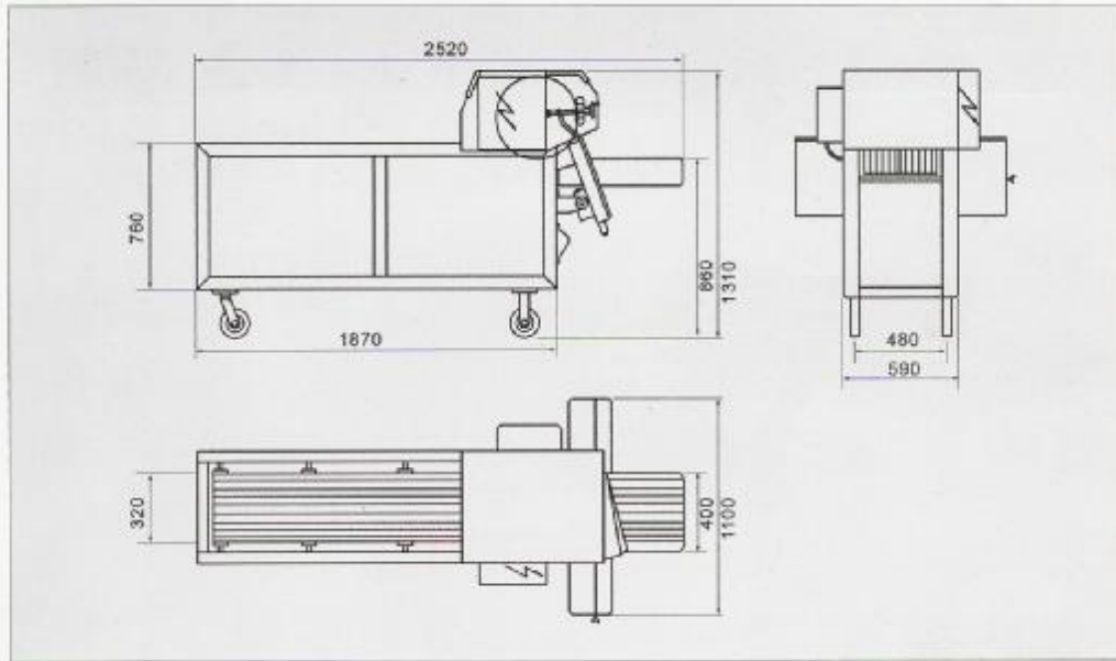
外形尺寸图 Main Dimension of Skinning Machine
